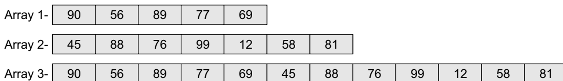
Figure 3.18 Merging of two unsorted arrays
