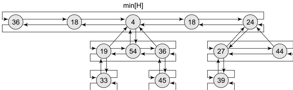
Figure 12.27 Linked representation of the Fibonacci heap shown in Fig. 12.24
