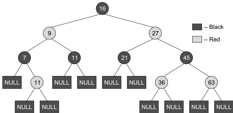
Figure 10.55 Red-black tree
