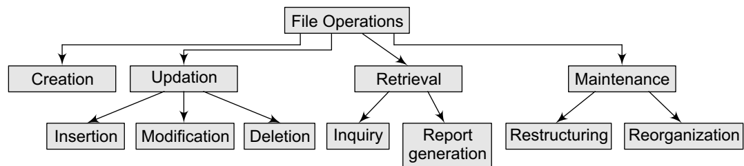
Figure 16.2 File operations
