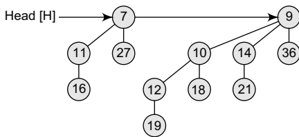
Figure 12.13 Binomial heap
