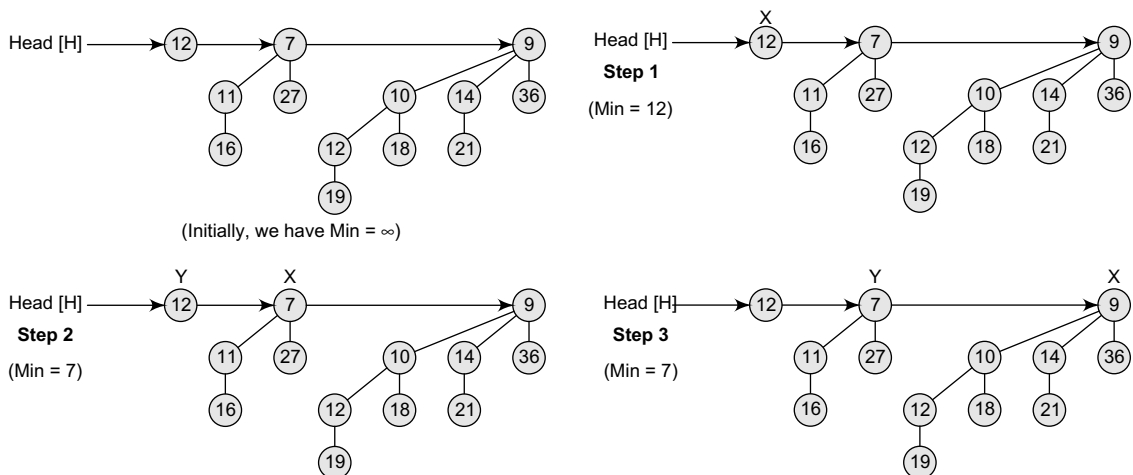
Figure 12.16 Binomial heap
