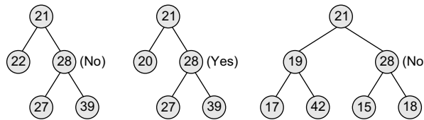
Figure 10.3 Binary trees
