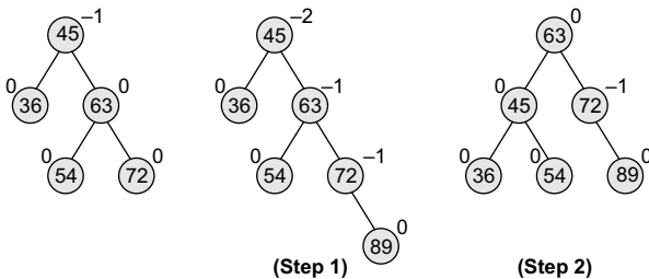
Figure 10.43 AVL tree
