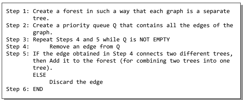
Figure 13.33 Kruskal's algorithm
