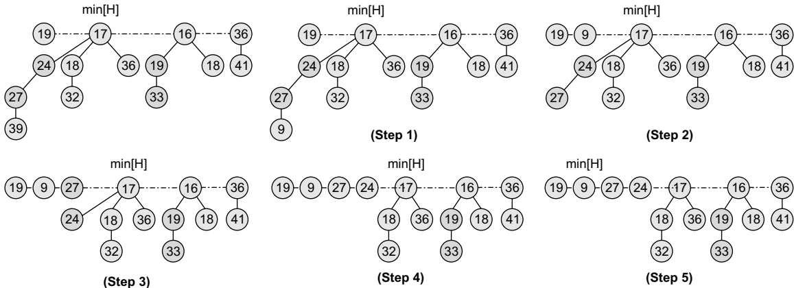
Figure 12.38 Fibonacci heap
